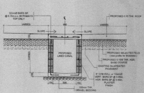
INTERIOR ROADS SECTION DETAIL OF LINE CANAL SCALE 1:20MTS
