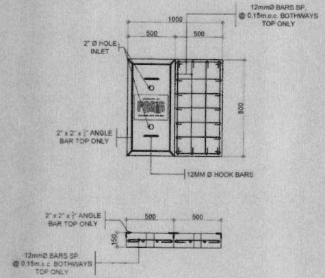
INTERIOR ROADS MANHOLE COVER DETAIL SCALE 1:20MTS
