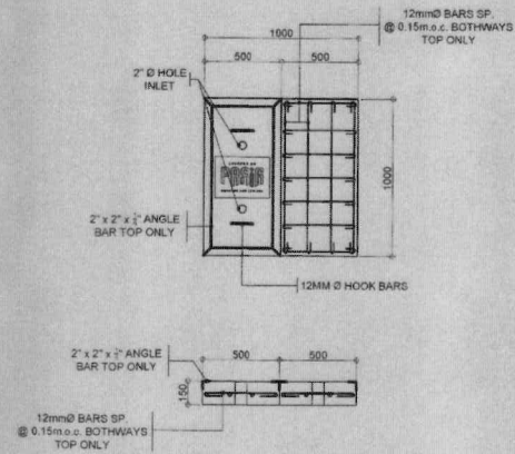
MAIN ROADS MANHOLE COVER DETAIL SCALE 1:20MTS
