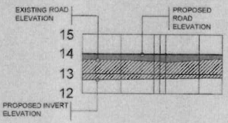
ROAD PROFILE
