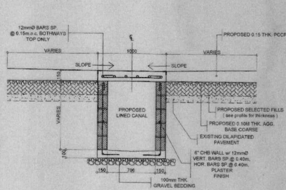
MAIN ROADS SECTION DETAIL OF LINE CANAL SCALE 1:20MTS
